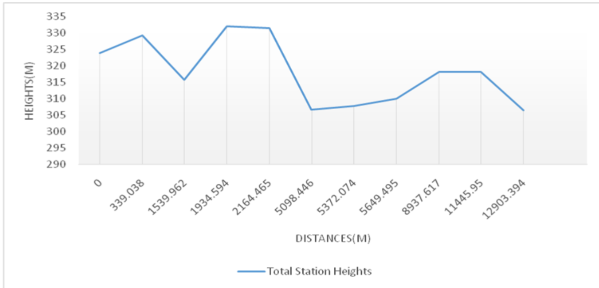
Figure. 3 Graph of Total Station Heights against Distance
