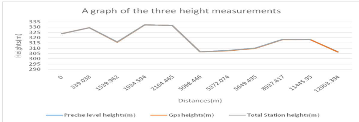
Figure. 5 Graph showing the three Height Measurements
