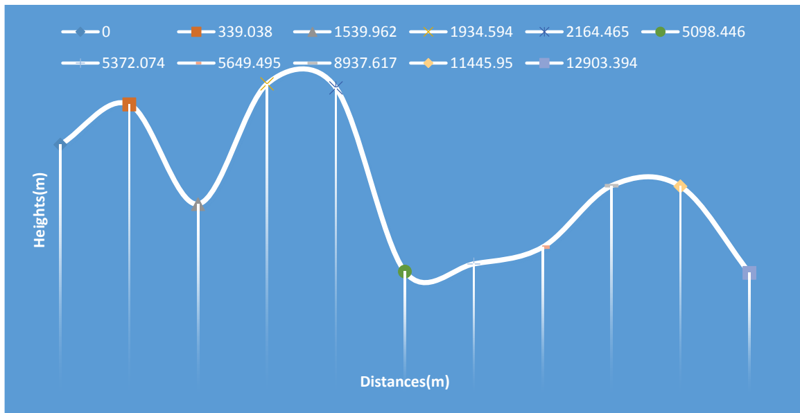
Figure. 2 Graph of GPS Heights against Distance
