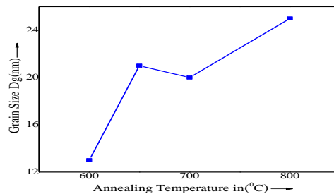
Figure 5. Change of Grain Size with different annealing temperature for the sample with composition Fe 73.5 Au 1 Nb 3 Si 13.5 B 9
