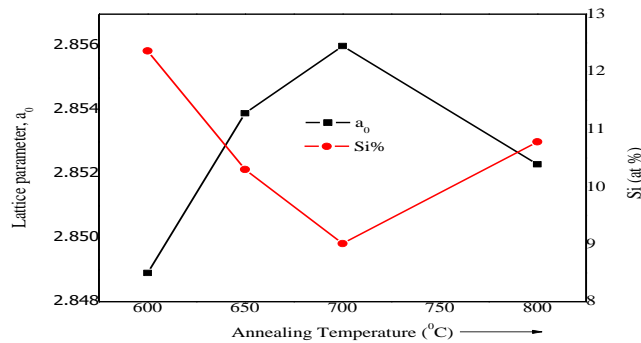
Figure 4. Change of Si (at. %) content and Lattice Parameter with different annealing temperature for the sample with composition Fe 73.5 Au 1 Nb 3 Si 13.5
