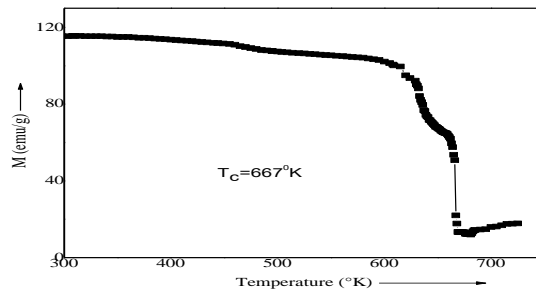
Figure 7 (a) Temperature dependence of specific magnetization of amorphous nanocrystalline ribbons with composition Fe_{73.5}Au_1Nb_3Si_{13.5}B_9 alloy
