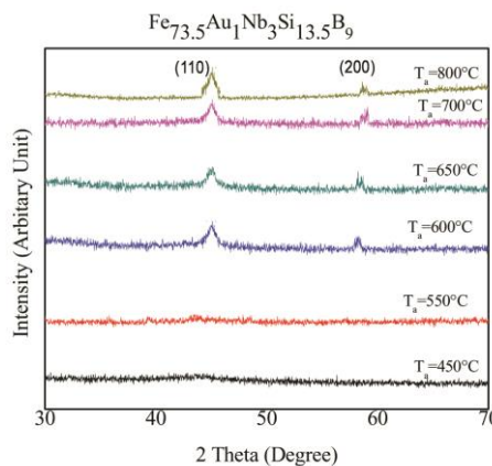
Figure 3. XRD spectra of Fe_{73.5}Au_1Nb_3Si_{13.5}B_9 alloys of annealed at different temperatures at constant annealing time 30 minutes
