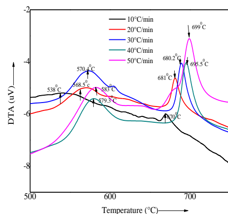
Figure 1(f) Effects of heating rate on DTA traces of nanocrystalline amorphous ribbon with composition Fe_{73.5}Au_1Nb_3Si_{13.5}B_9 at the heating rate of 10^\circ C to 50^\circ C /min
