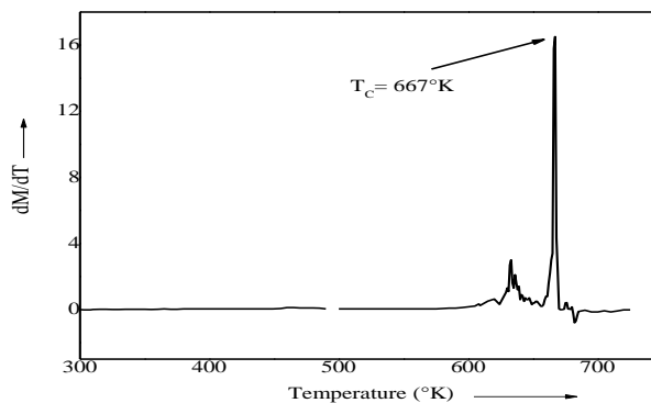
Figure 7(b) \frac{dM}{dT} versus temperature curve of amorphous Nanocrystalline ribbons with composition Fe_{73.5}Au_1Nb_3Si_{13.5}B_9 alloy.
