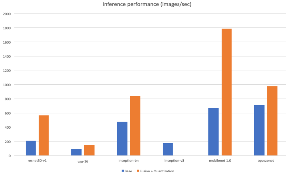
Figure 3: Performance Comparison for INT8 inference
