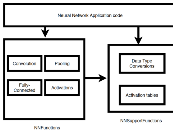
Figure 4: CMSIS-NN Library
