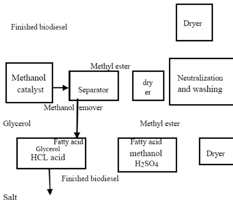
Figure1: Schematic diagram of biodiesel production
