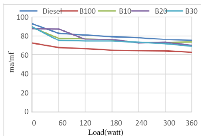
Figure 6: Air fuel ratio Vs Load
