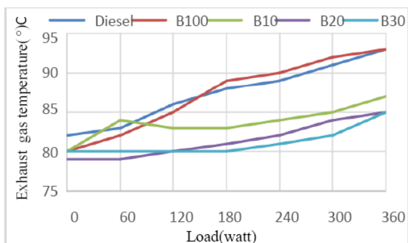
Figure 3: Exhaust gas temperature Vs Load
