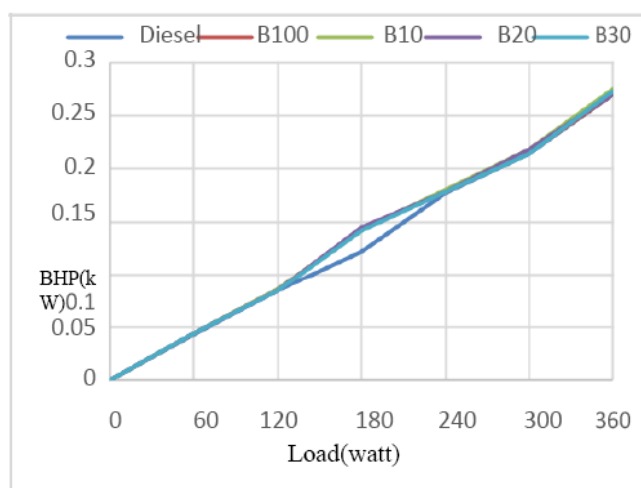
Figure 5: BHP Vs Load
