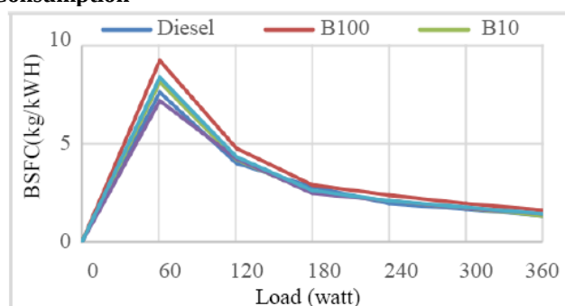
Figure 4: Break Specific fuel consumption Vs Load
