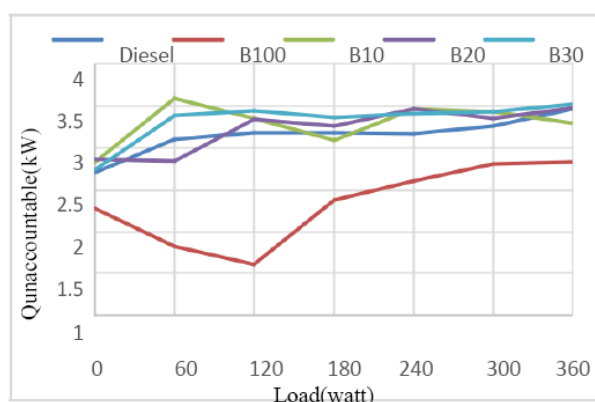
Figure 7: Unaccountable heat (Q) Vs Load
