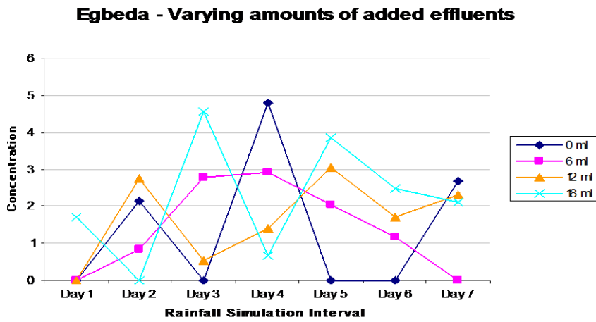
Figure 4: Copper concentrations (mg/l) with Rainfall Simulation Interval for varying effluent proportions.
