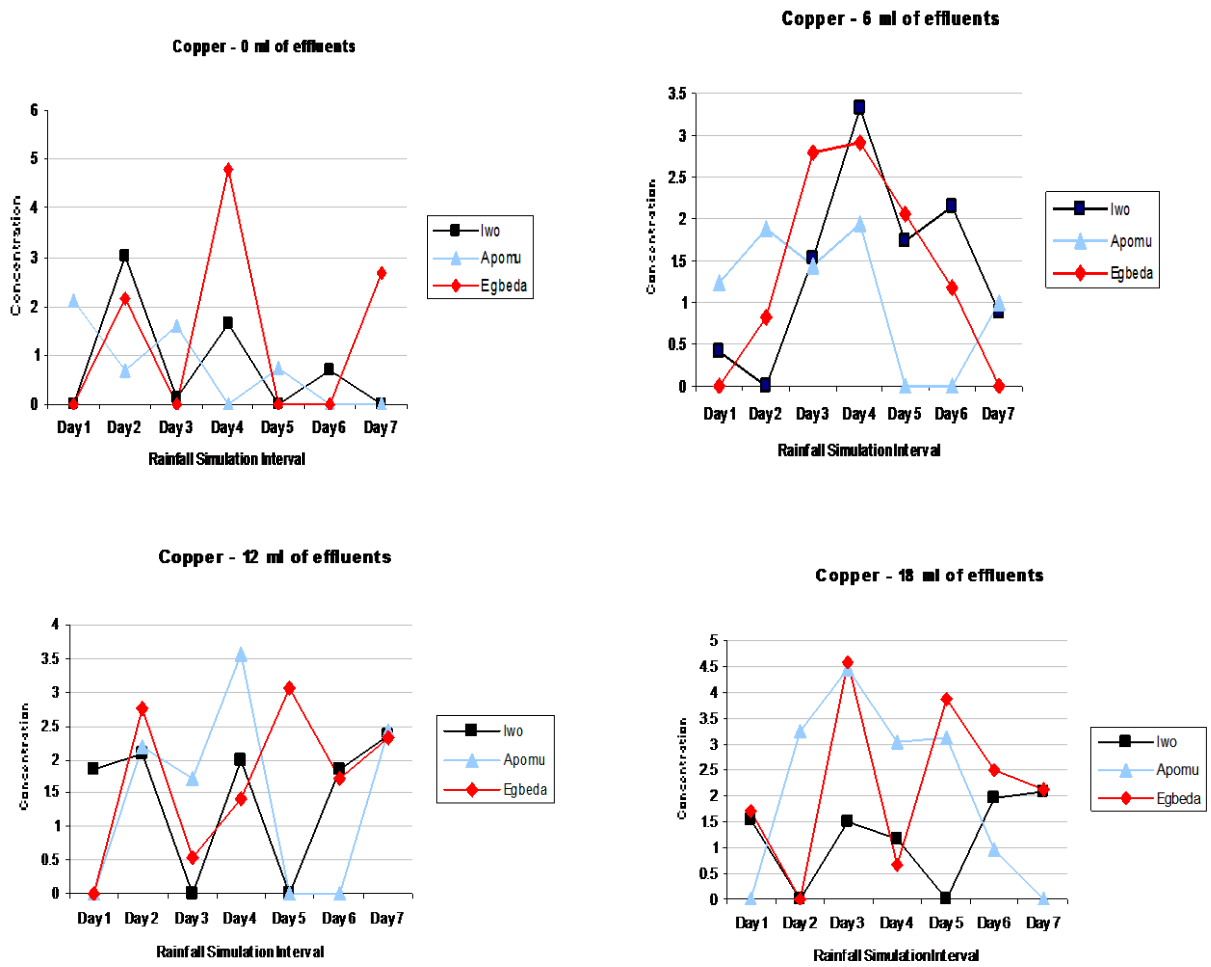
Figure 2: Concentrations (in mg/l) of Copper with Rainfall Simulation Interval for different soil
