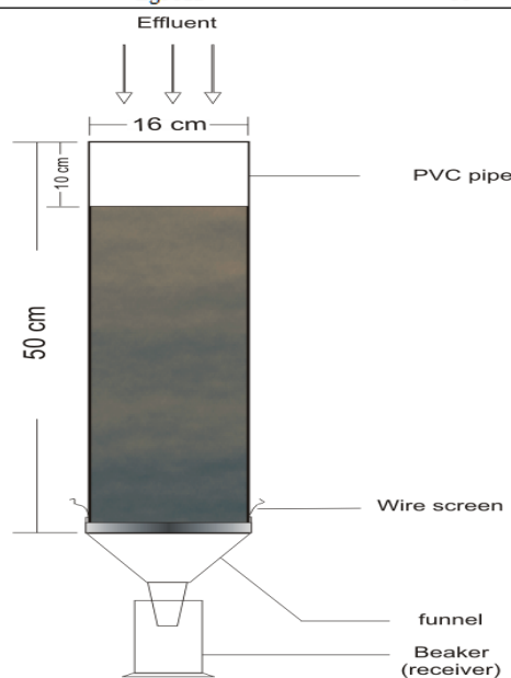
Fig. 1: Soil column set-up with receiver in place
