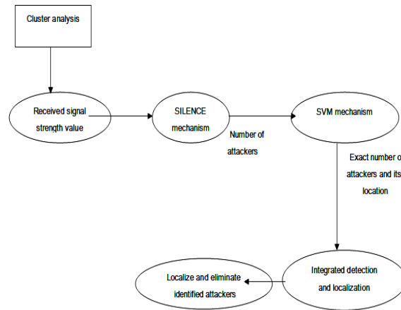
Fig 1.Overall working view of the system
