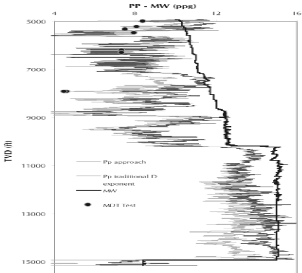
Figure 6. Pore pressure well 10 with pressure test
