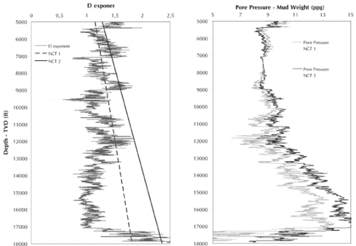
Figure 1. A. user-defined normal Compaction Trends (NCT). B. Variation of pore pressure calculated with several Normal Compaction Trends (NCT)
