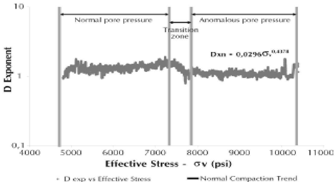
Figure 4. D exponent versus effective stress for all data points available in the field. Note that the NCT of the field is represented by the trend line fit to data from the upper Carbonera Formation
